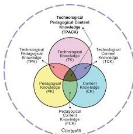
Figure 1. TPACK Model
